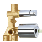
KB111034 3 Inlet Diverter Body (47 mm)
